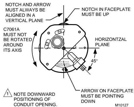
Fig. 6. C7061 mounting positions.
