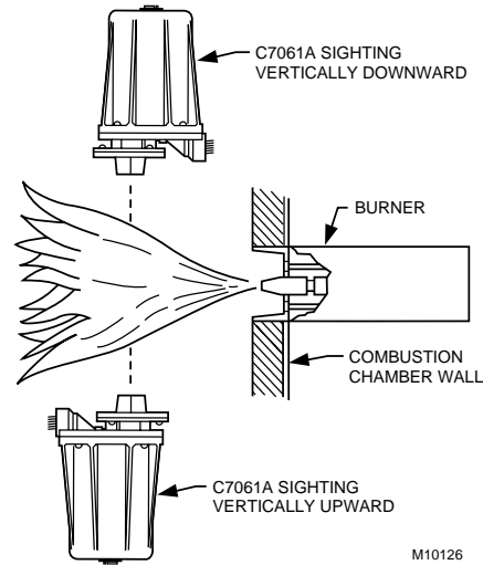
Fig. 5. Vertical mounting of C7061A.
