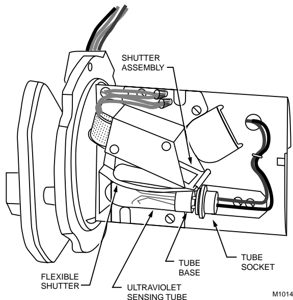
Fig. 11. Replacing ultraviolet radiation sensing tube.
