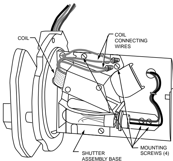
Fig. 12. Replacing coil and shutter assembly.
