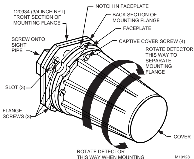
Fig. 7. Mounting C7061A Detector.
