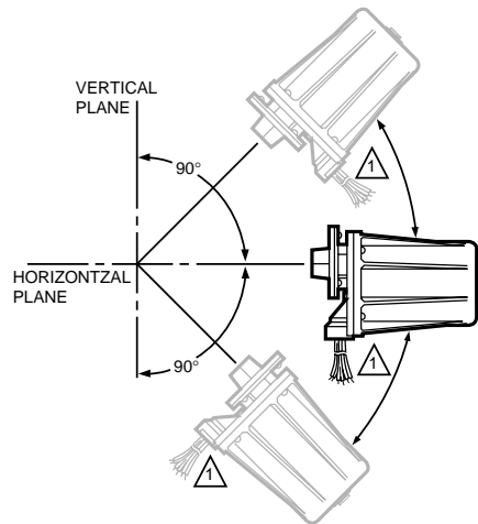
Fig. 5. Vertical mounting of C7061A.
