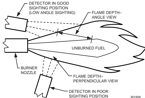
Fig. 2. Detector sighting angle.
