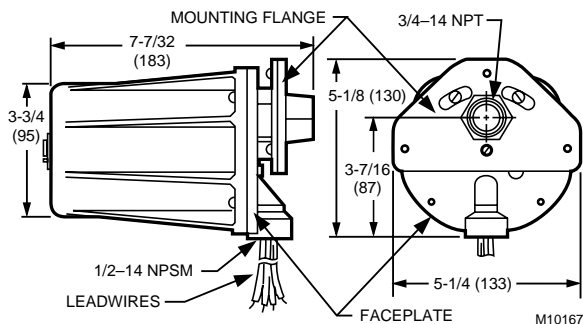
Fig. 1. Dimensions of C7061A in in. (mm).
